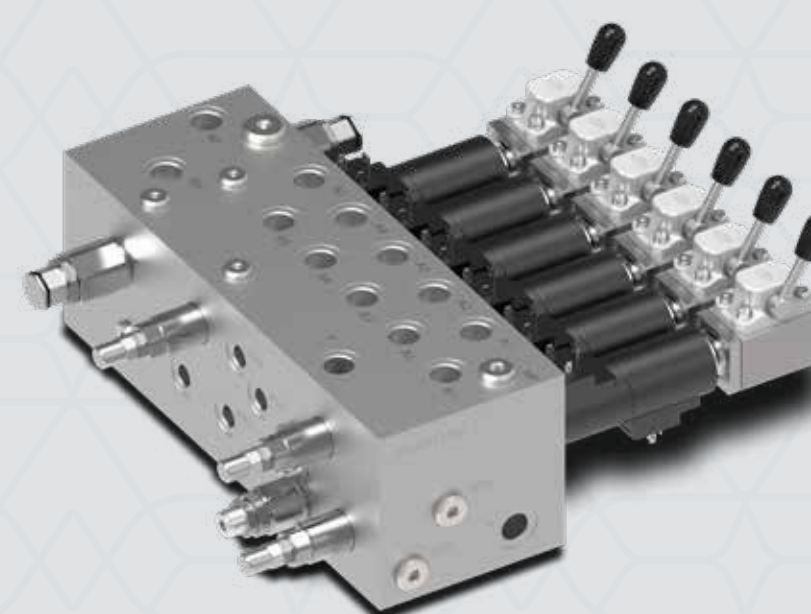
HIC Hydraulic Integrated Circuit
