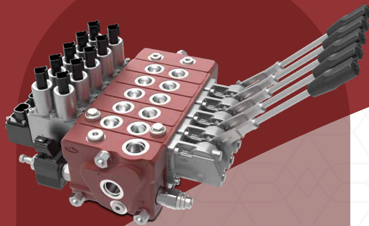
DPX100 Full Flow Sharing directional control valve
